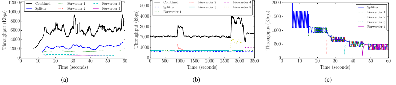
Fig. 6. Simulation results. (a) shows the throughput of individual forwarding nodes compared to the goodput of the system. (b) shows the distribution algorithm adjusting to forwarders connecting and disconnecting. (c) shows the throughput of all forwarders are equalized when new forwarders are added.
